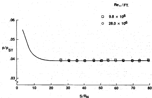
Fig. 2 Surface pressure data for the nonadverse pressure gradient model.
