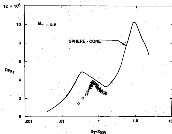
Fig. 3 Transition Reynolds numbers for the nonadverse pressure gradient mode.
